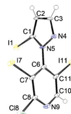
Fig. 4 ORTEP diagram (30% probability) of 9m .
